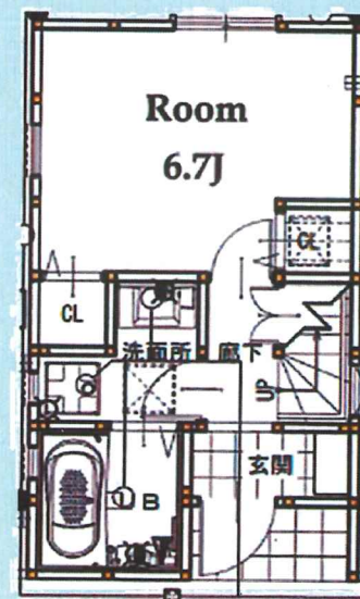
1階 [23.79㎡]
